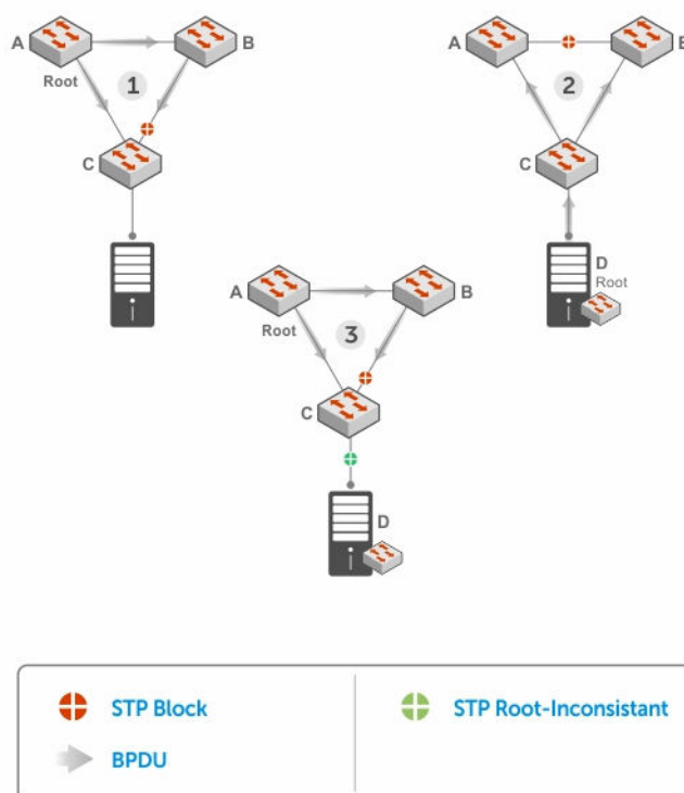
Figure 114. STP Root Guard Prevents Bridging Loops
